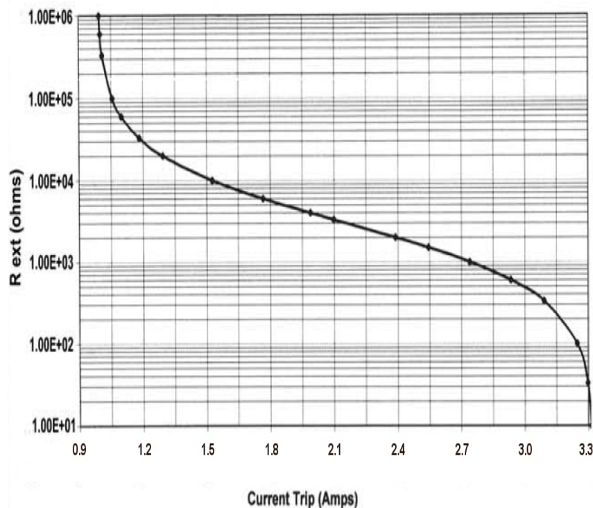
Figure 4 – SPDP03D270 Current Rating Trim Resistor Selection
