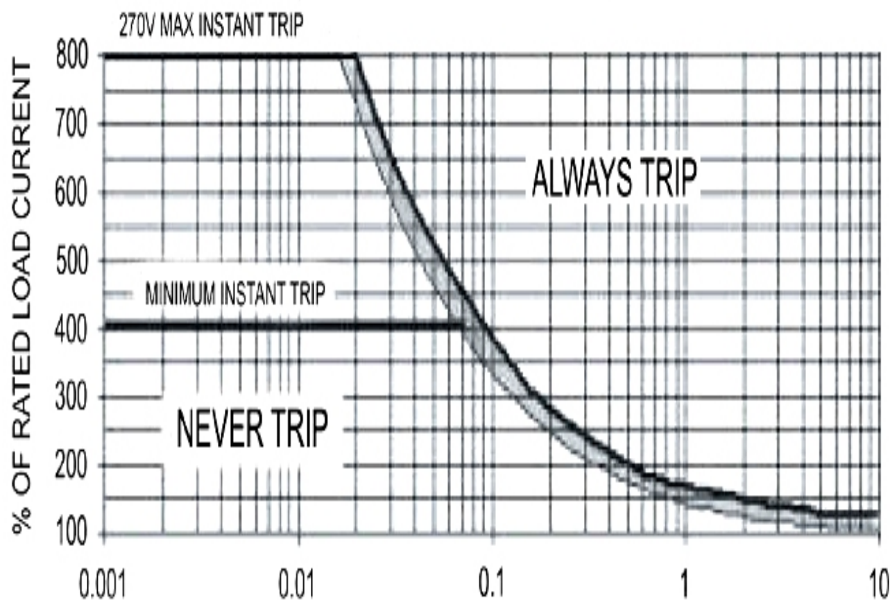
Figure 1 - Trip Curve
