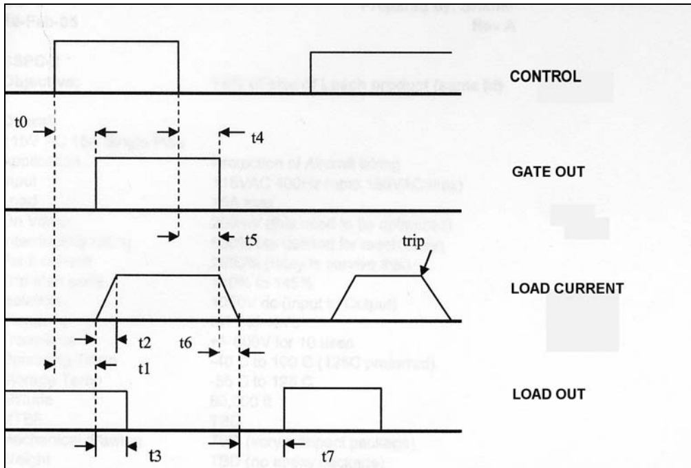
Figure 2 - Timing Diagram
